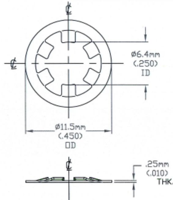
SIZE 6 RETAINER (SEE NOTE 1)
